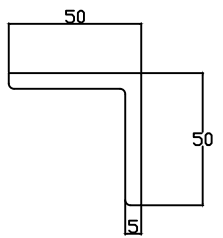
DETAIL A SCALE 1 : 3
