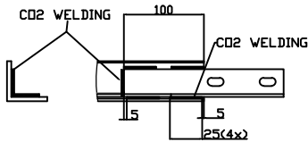
DETAIL A SCALE 2 : 15
